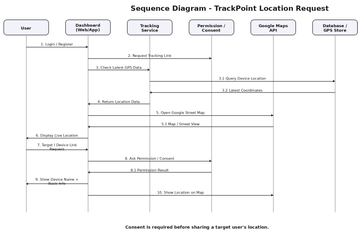
Figure 4 — Sequence Diagram: TrackPoint Location Request
