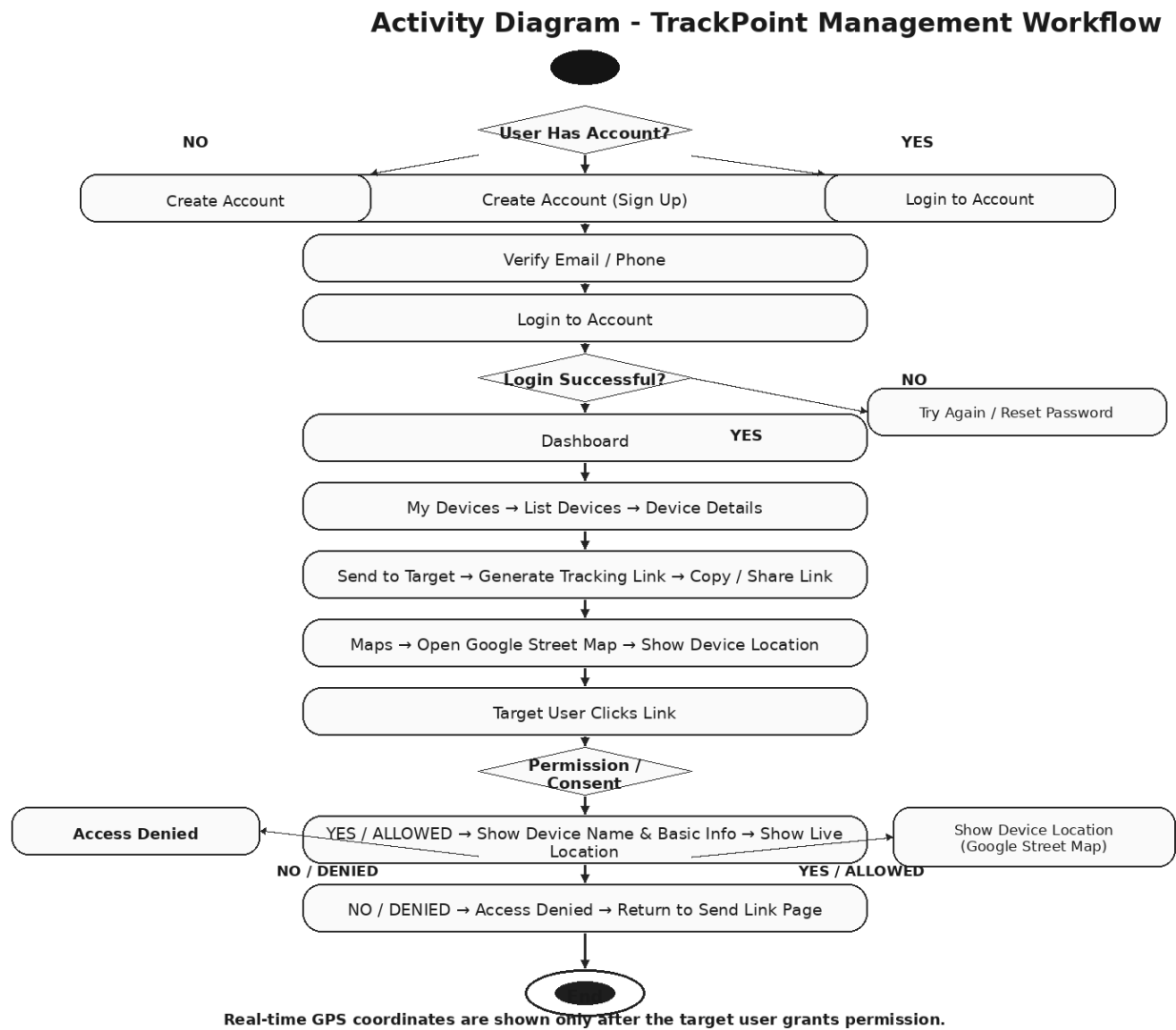
Figure 3: Activity diagram showing the end-to-end TrackPoint workflow, including account handling, dashboard access, device/link operations, map visualization and permission-controlled location disclosure.
